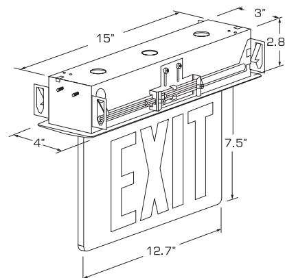
Recessed Ceiling
